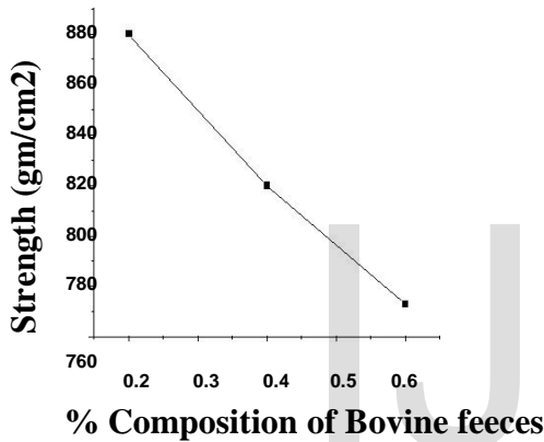
Fig. 4 Shows the Green compression strength of UFS.
