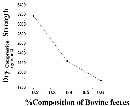
Fig. 5 Shows the Dry compression strength of UFS.
